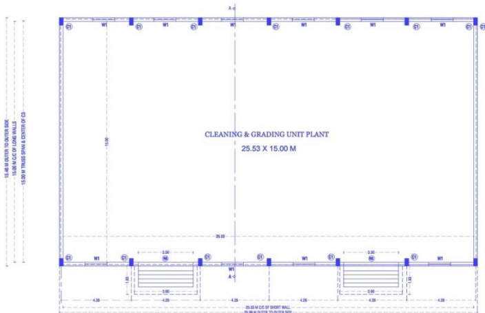
CLEANING & GRADING UNIT PLANT PLAN
